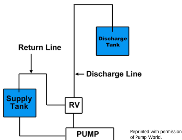
Figure 7.7.5. Schematic of pump and relief valve.
