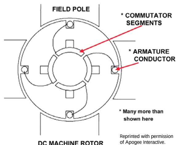
Figure 7.9.3. Parts of a direct current motor. 20
