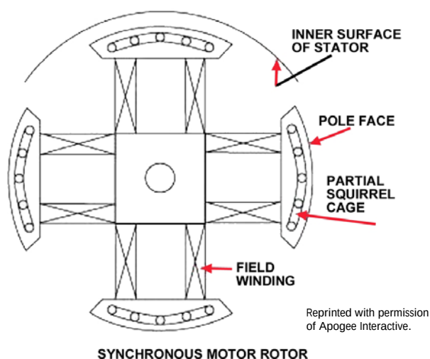
Figure 7.9.4. Parts of an alternating current motor.
