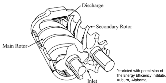
Figure 7.10.3. Helical-lobe rotors.
