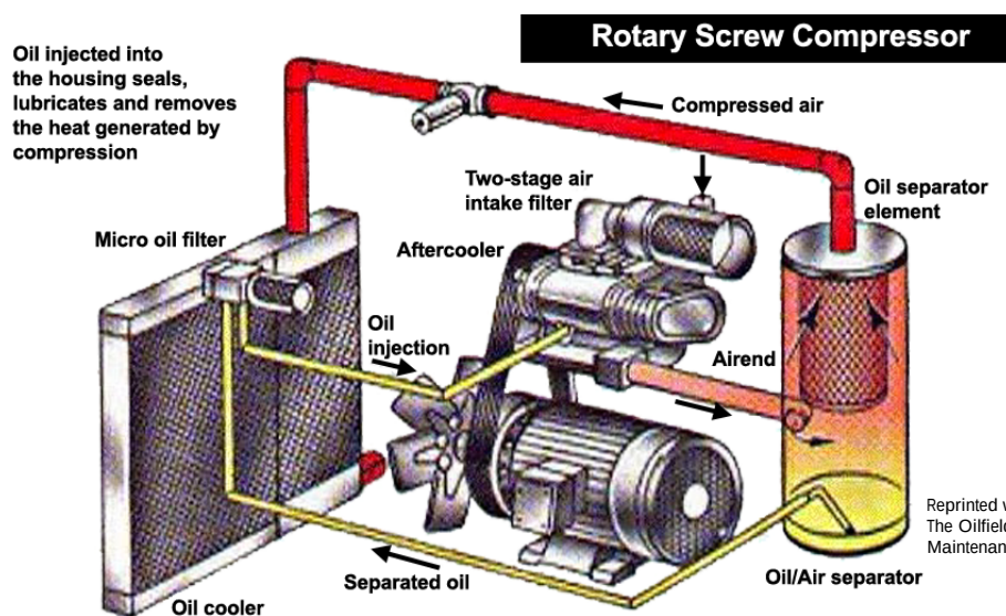
Figure 7.10.1. Rotary screw compressor.
